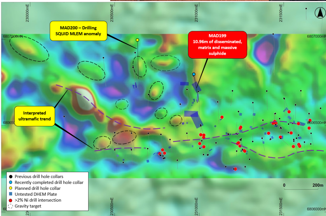
Plan view map of West End and Investigators showing recent gravity survey data (25m spacing) and prior drilling. Gravity highs are targets for potential areas of nickel-copper sulphides.
