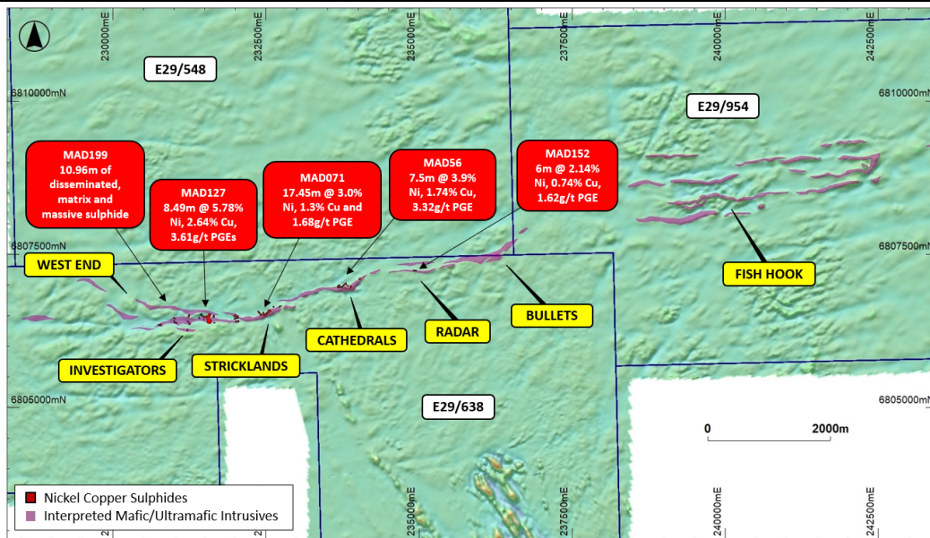
Map (against magnetic RTP 1VD data) showing intrusives along the Cathedrals Belt and highlighting the continuation of high grade mineralisation to the west
